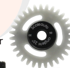
SC-1171R Polyamide Anglewinder Gear 31 th M50 for 2.38mm axle diam 17mm. M2,5 screw
