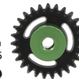
SC-1167BR Polyamide Anglewinder Gear 27th M50 for 2.38mm axle. \varnothing 15.8mm. Screw M2.5 Reverse Insert.
